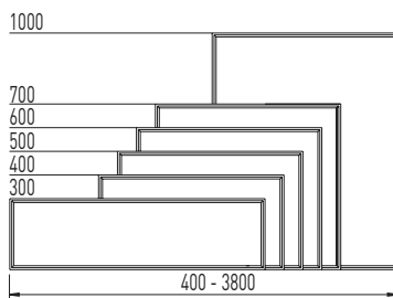
Fionia 68, profile
