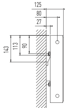
Fionia 98, profile
