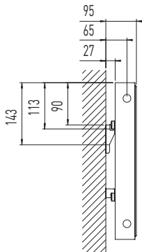
Fionia 68, profile
