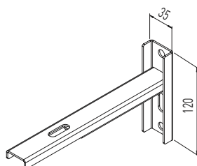
Bracket BPH for P100/184
