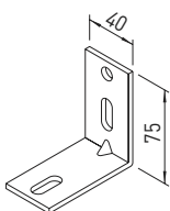
Bracket BPH for P100/100
