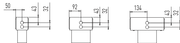
P100/100, 184 and 268. Tappings E-F/F-E
