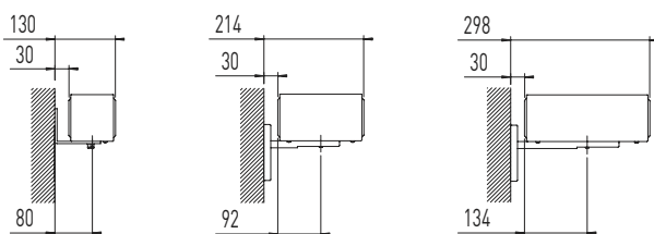
P100/100, 184 and 268. Tappings E-F/F-E
