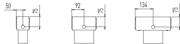
P100/100, 184 and 268. Tappings B-B/D-D
