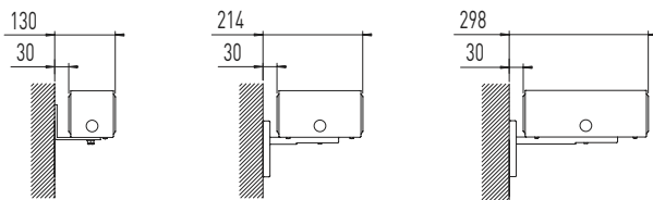
P100/100, 184 and 268. Tappings B-D/D-B
