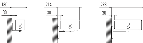
P100/100, 184 and 268. Tappings B-B/D-D
