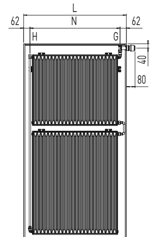
Built-in valve format 3 (top), rear view
