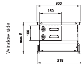
Cross-section through trench height 150/200 mm (example shown with roll-up grille)
