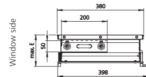
Cross-section through trench height 92/120 mm (example shown with roll-up grille)
