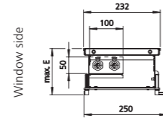
Cross-section through trench height 92/120 mm (example shown with roll-up grille)
