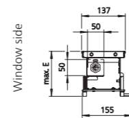
Cross-section (Example with roll-up grille)
