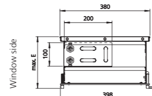
Cross-section through trench height 150/200 mm (example shown with roll-up grille)
