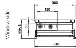
Cross-section through trench height 92/120 mm (example shown with roll-up grille)
