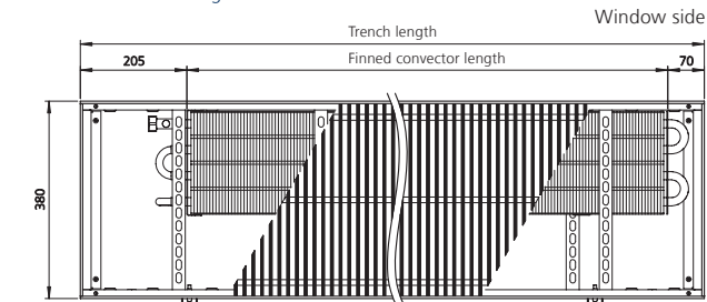
Top view of trench height 150/200 mm (view without cover panel) Room side
