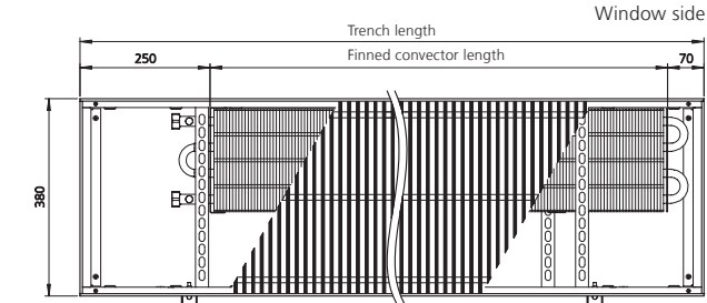
Top view of trench height 92/120 mm (view without cover panel) Room side
