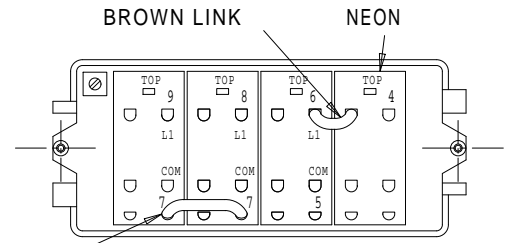
BROWN LINK REAR VIEW OF SWITCH ASSY. IN REMOTE CONTROL BOX
